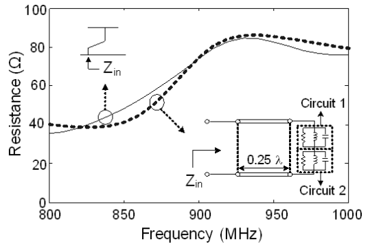
(a) 저항 (a) Resistance
