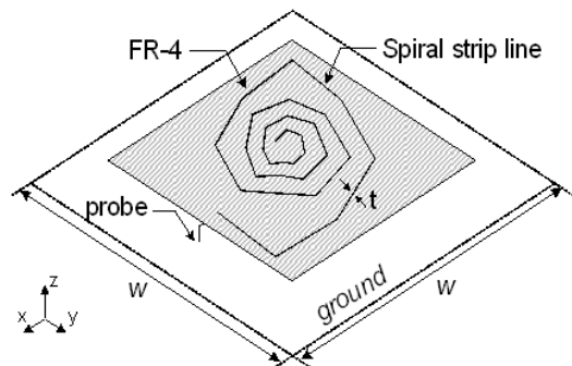
(c) 사시도 (c) Perspective view
